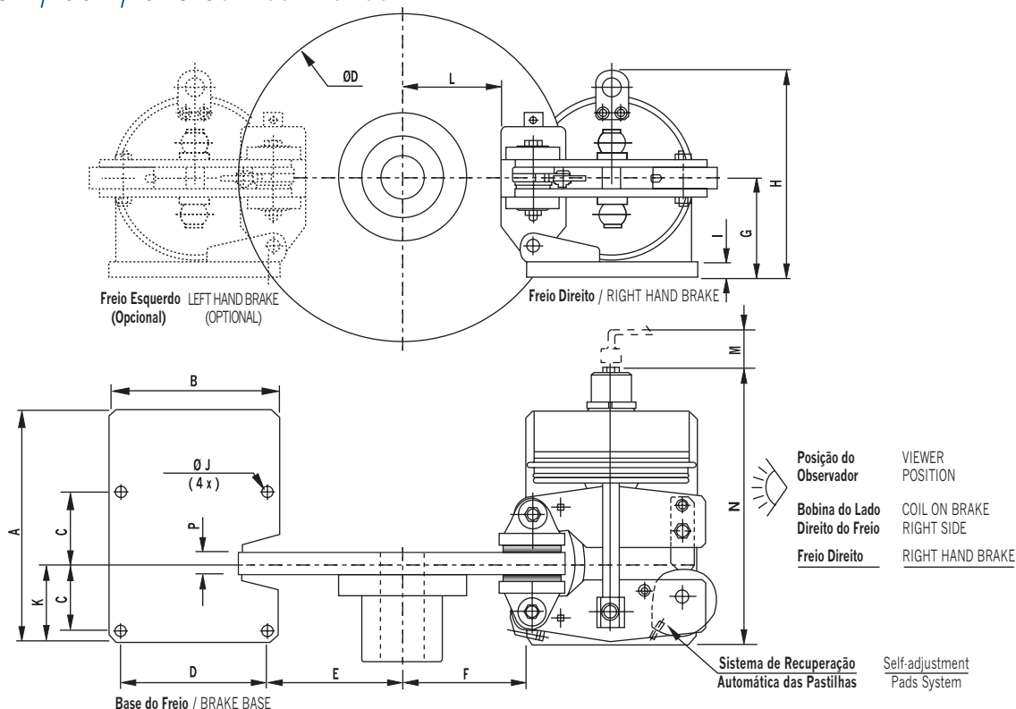
Freio 5CR - Peso: 55 [kgf] / 5CR Brake - Weight: 55 [kgf]
