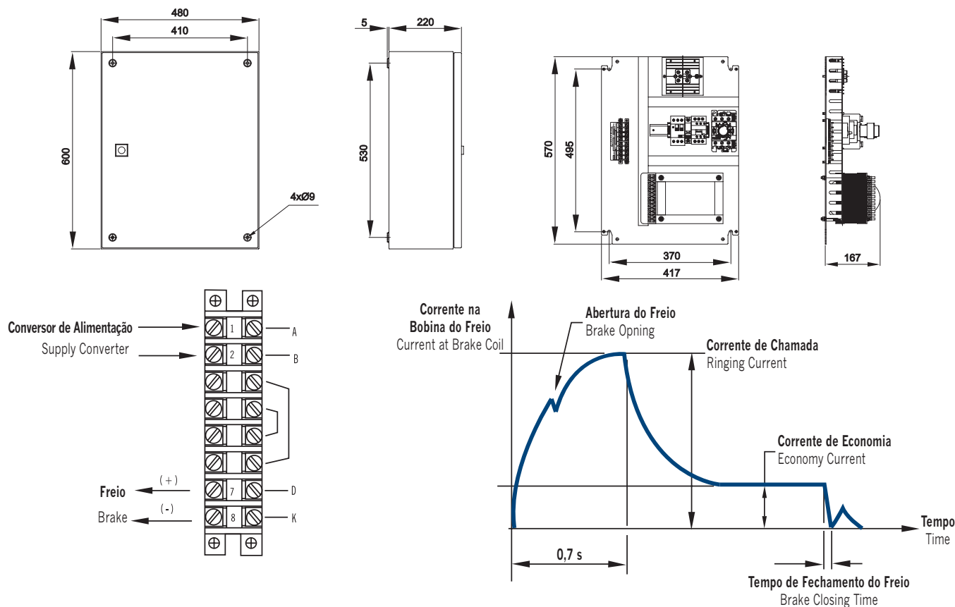
Características do Conversor C-2200-CE3 / Features of Converter C-2200-CE6
